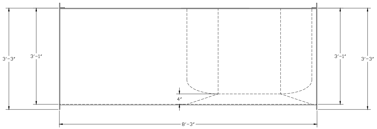
ELEVATION VIEW
