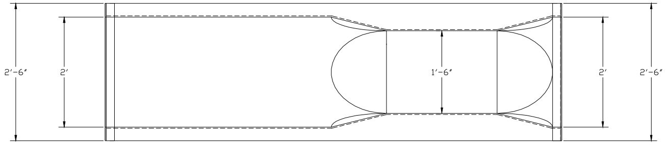
PLAN VIEW
