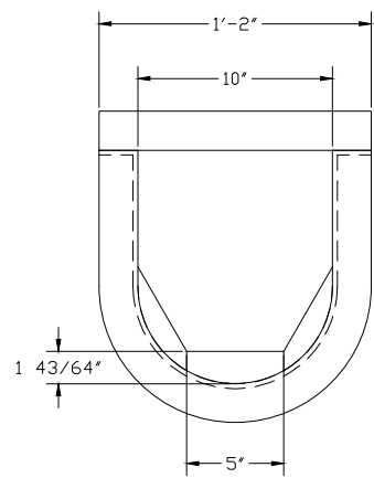
DISCHARGE ELEVATION
