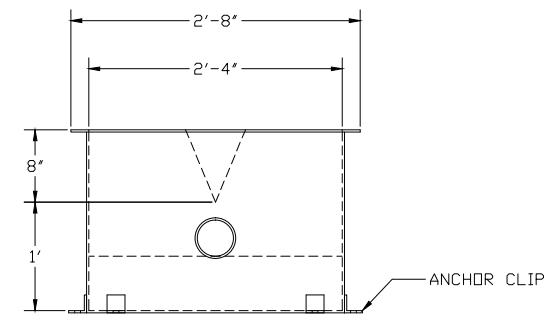
DISCHARGE ELEVATION VIEW
