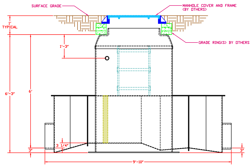
ELEVATION VIEW
