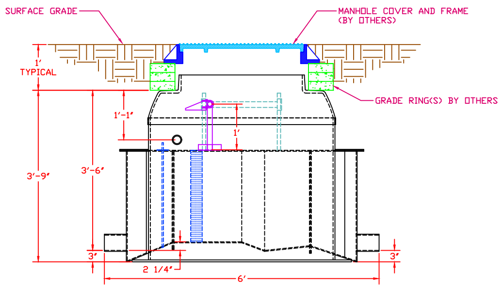
ELEVATION VIEW
