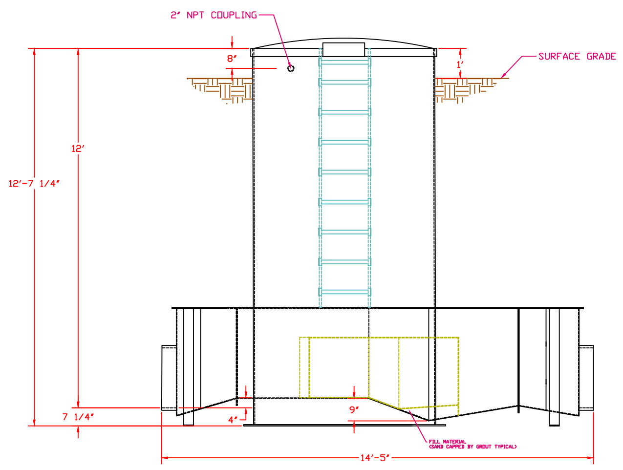
ELEVATION VIEW
