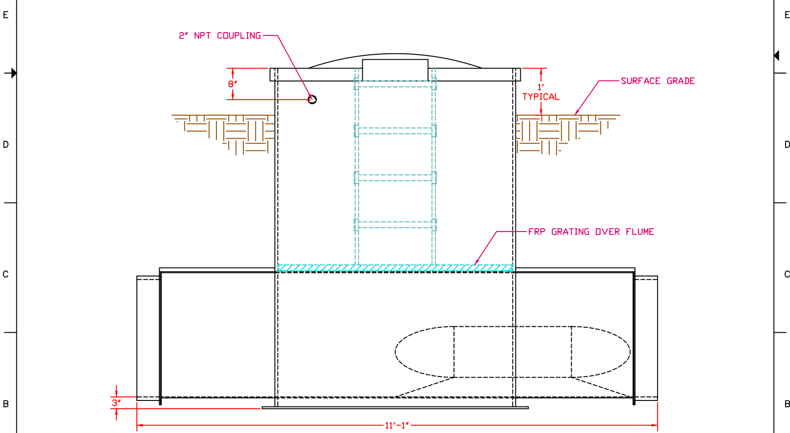
ELEVATION VIEW
