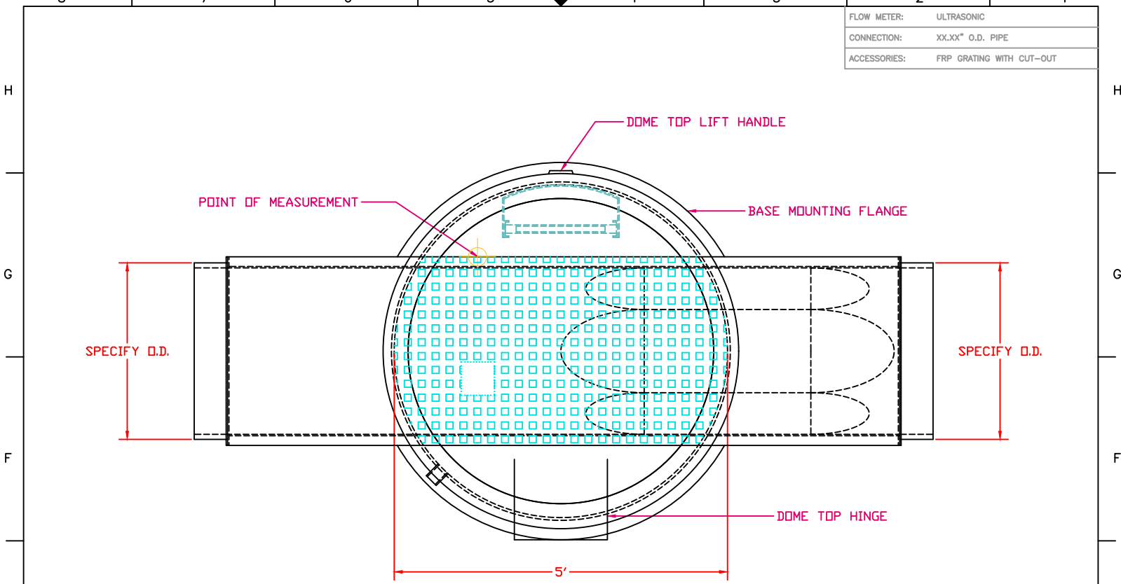
PLAN VIEW
