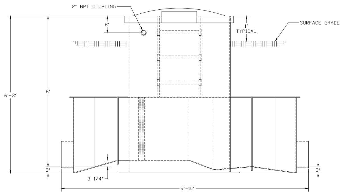
ELEVATION VIEW
