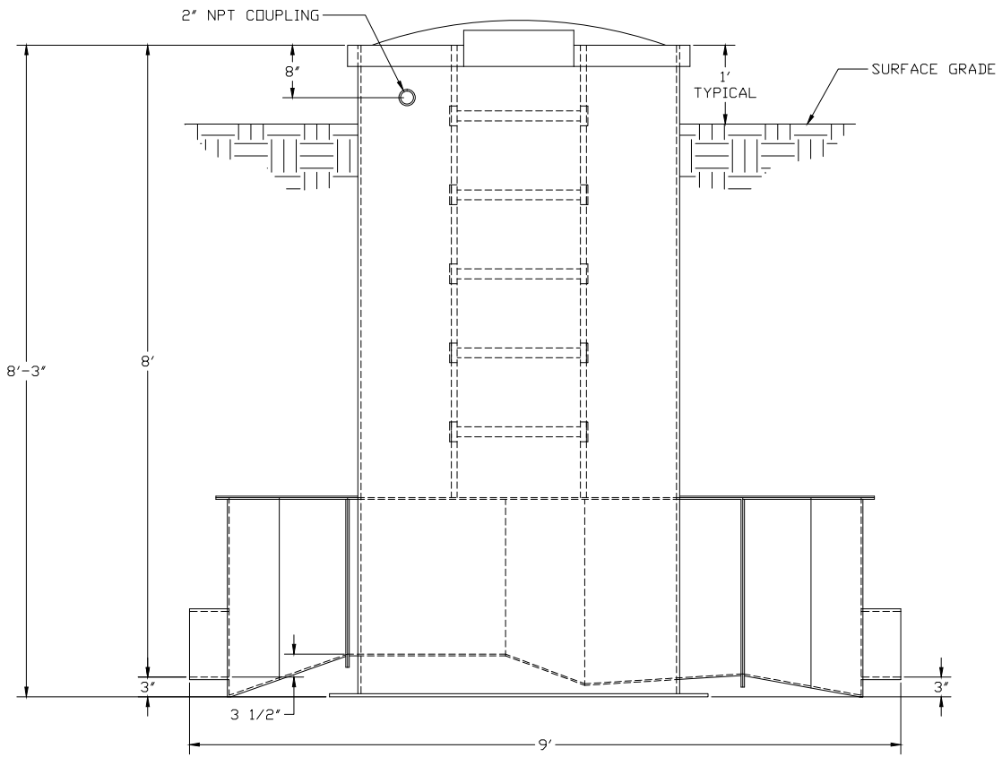
ELEVATION VIEW
