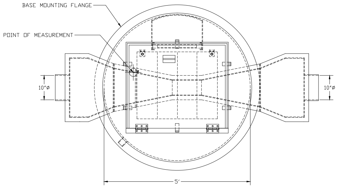
PLAN VIEW
