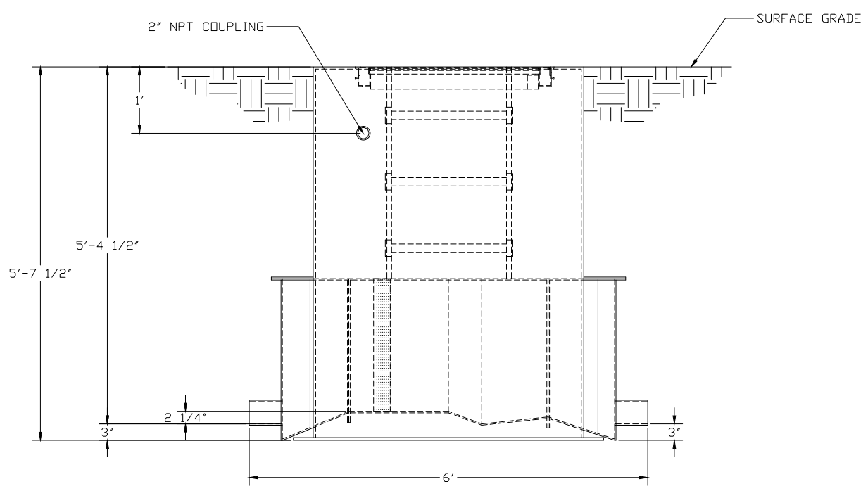
ELEVATION VIEW
