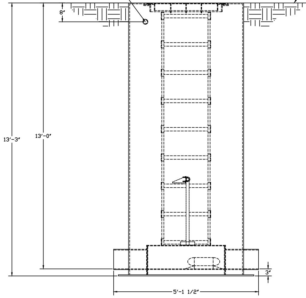
ELEVATION VIEW
