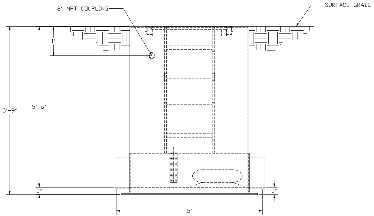
ELEVATION VIEW
