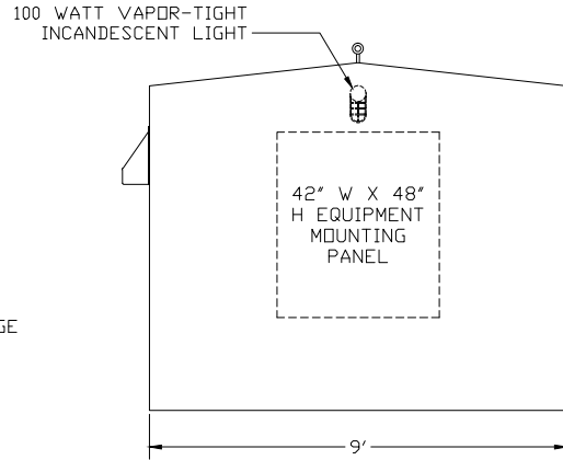
REAR ELEVATION
