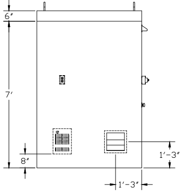
LEFT ELEVATION
