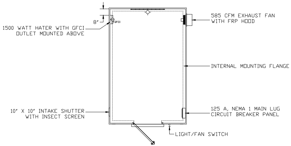
PLAN VIEW
