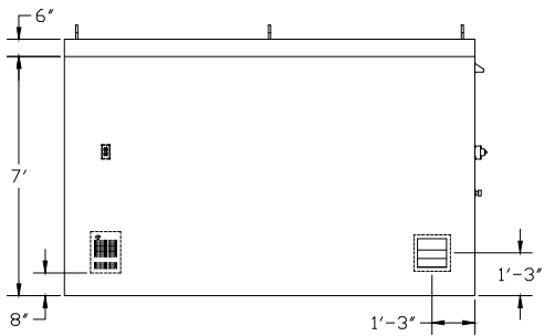
LEFT ELEVATION
