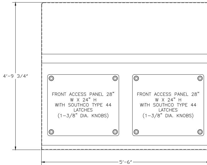
FRONT ELEVATION
