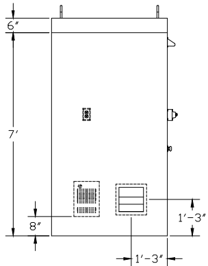
LEFT ELEVATION
