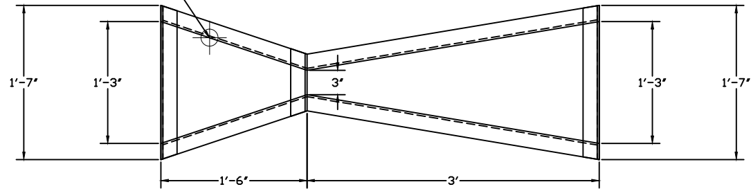
PLAN VIEW
