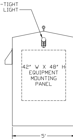
REAR ELEVATION
