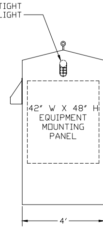
REAR ELEVATION
