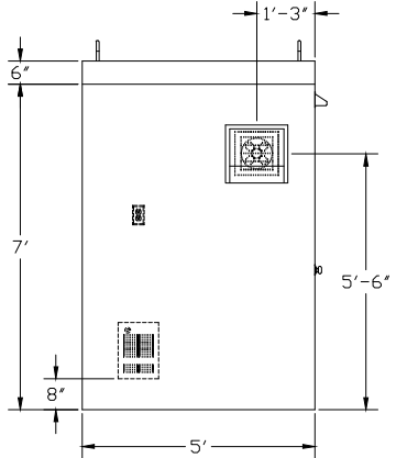
LEFT ELEVATION
