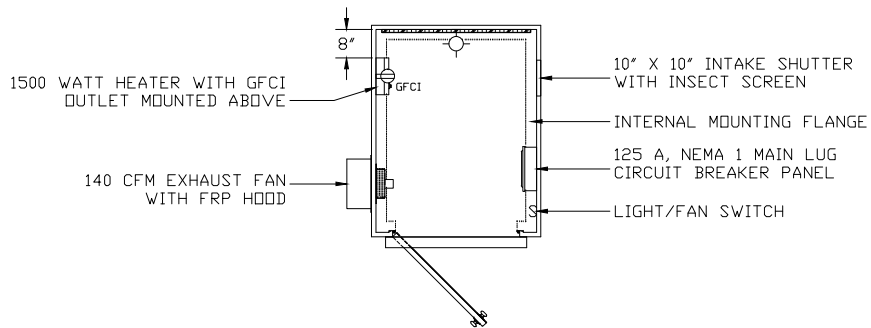
PLAN VIEW
