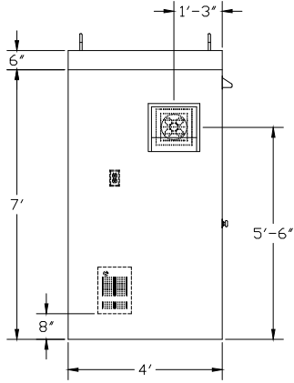
LEFT ELEVATION
