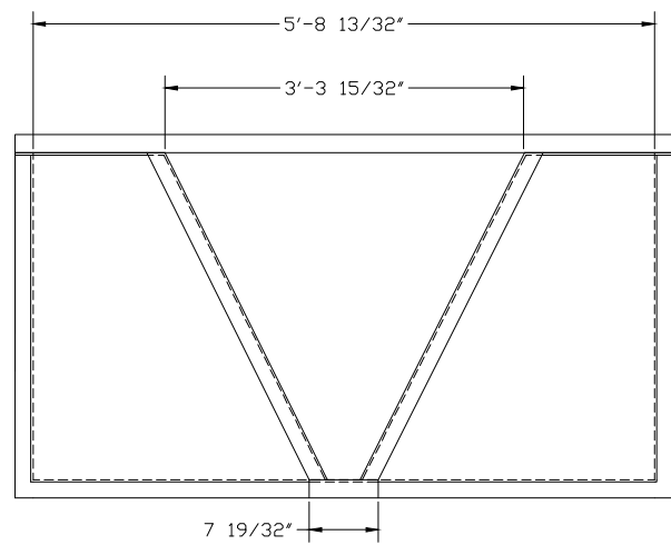
DISCHARGE ELEVATION
