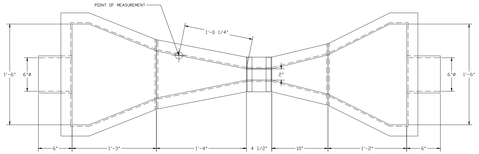
PLAN VIEW
