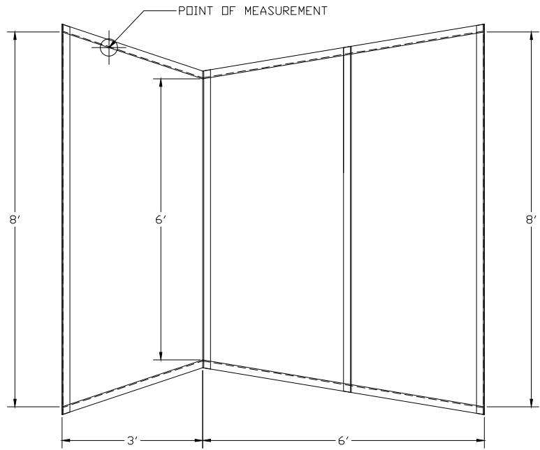
PLAN VIEW
