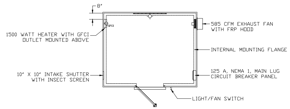
PLAN VIEW
