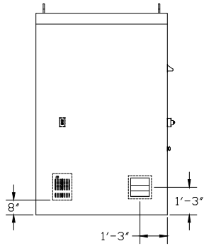
LEFT ELEVATION
