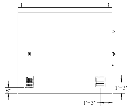
LEFT ELEVATION
